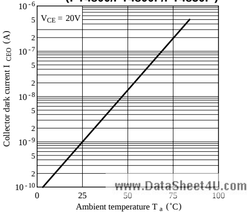
Fig. 2-a Collector Dark Current vs. Ambient Temperature (PT4800/PT4800F/PT4850F)
