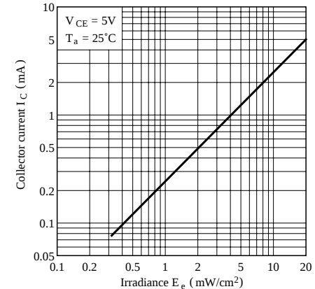
Fig. 4-b Collector Current vs. Irradiance
