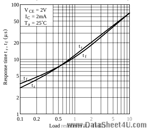
Fig. 7-a Response Time vs. Load Resistance
