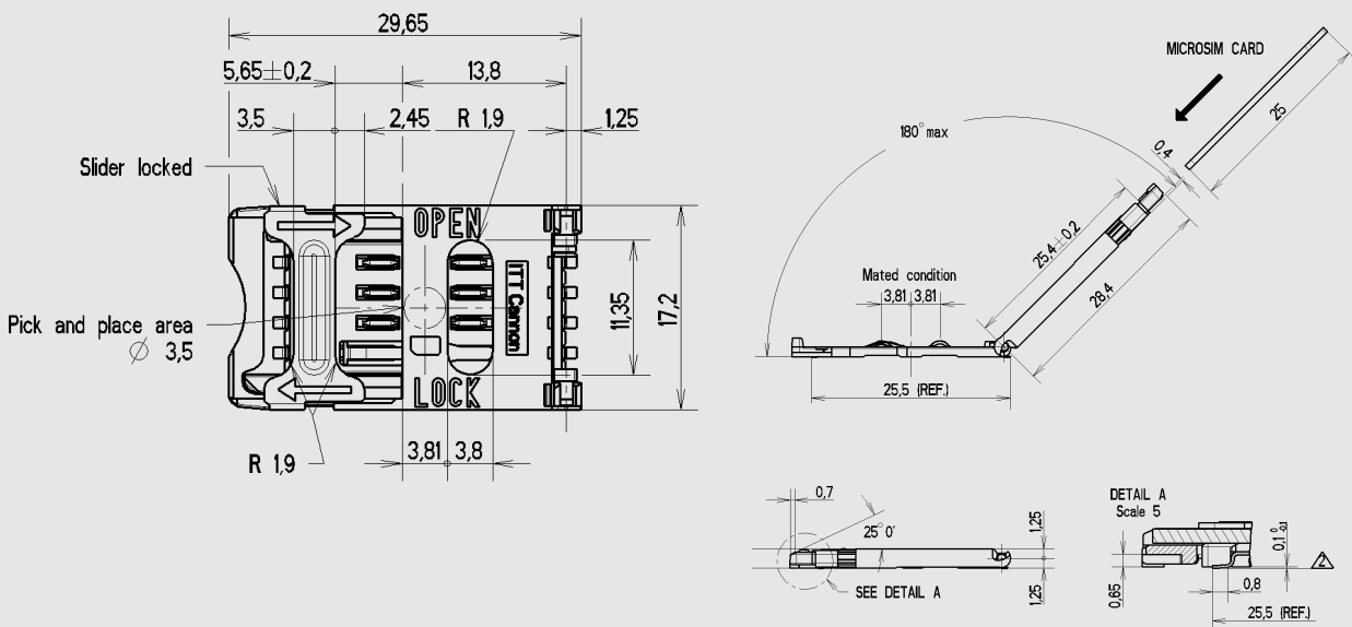
Hinged Cover CCM03-3013 (6 contacts + Card Detect Switch)
