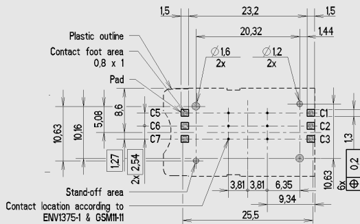
RECOMMENDED PC BOARD LAYOUT (Component side)
