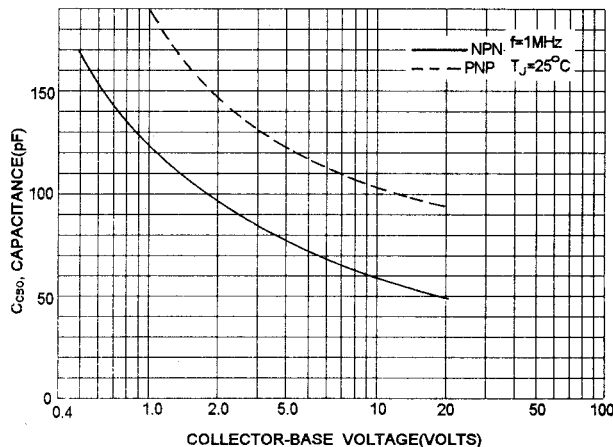
COLLECTOR-BASE CAPACITANCES
